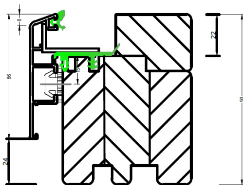
Premium Protect Classic
