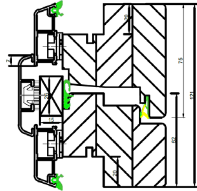
Premium Protect Classic Stulp
